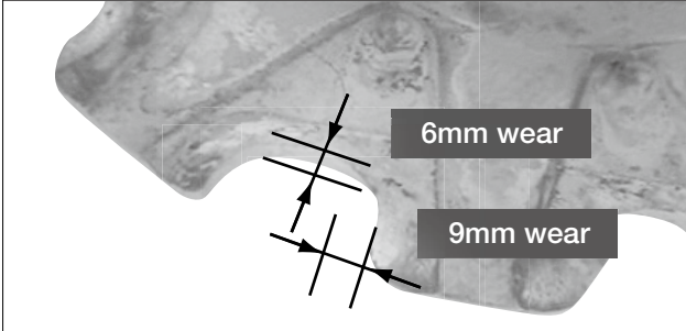
Previous Tooth Insert Sprockets (one year operation)
