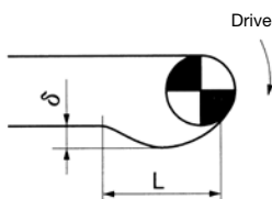
Chain slack ( \delta ) \cong 0.1L
