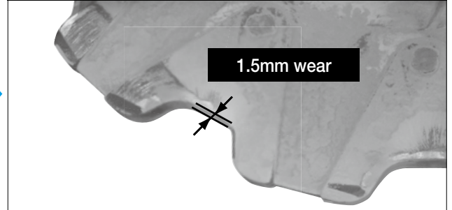
Thermally Sprayed Tooth Insert Sprockets (one year operation)
