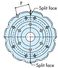
Ring Replaceable Teeth (D-split)
